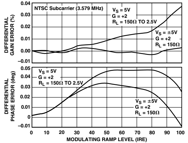
TPC 10. Differential Gain and Phase Errors
