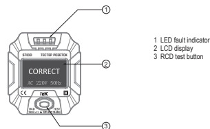
Socket tester ST03D
