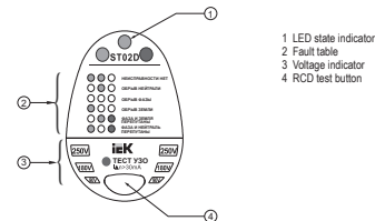
Socket tester ST02D
