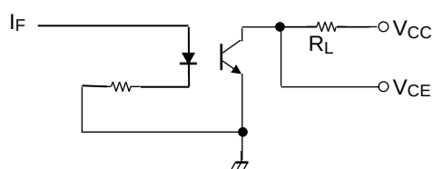
Figure 1: Switching Time Test Circuit
