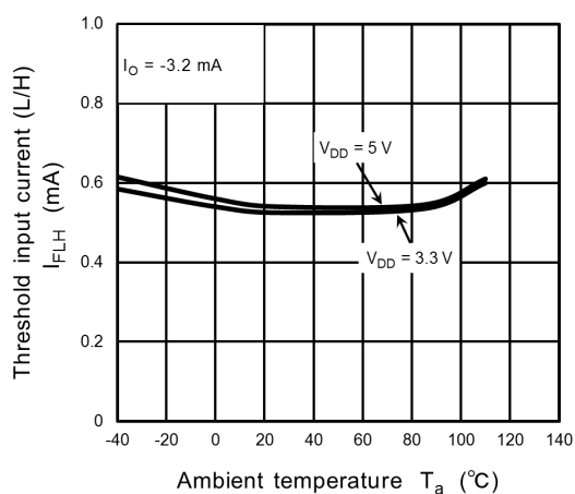
Fig. 13.2.9 I_{FLH} - T_a
