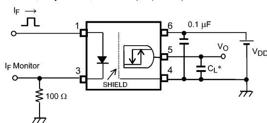
Fig. 13.1.6 Switching Time Test Circuit and Waveform
