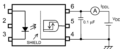
Fig. 13.1.3 IDDL Test Circuit
