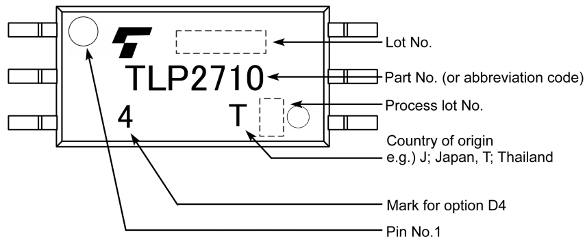
Fig. 17.4 Marking Example (Note)
