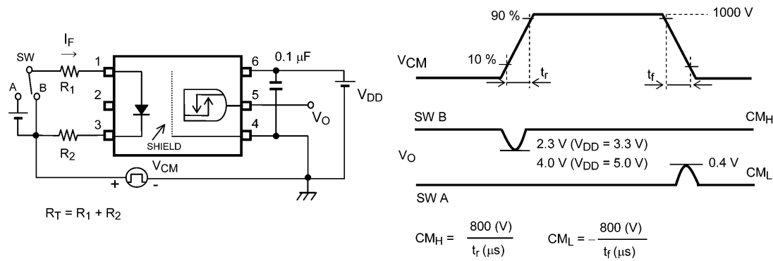
Fig. 13.1.7 Common-Mode Transient Immunity Test Circuit and Waveform
