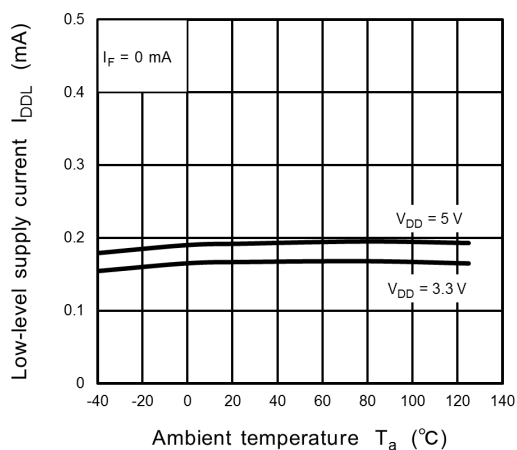
Fig. 13.2.7 I_{DDL} - T_a
