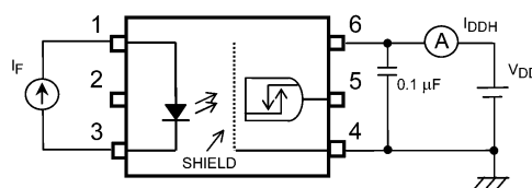
Fig. 13.1.4 IDDH Test Circuit
