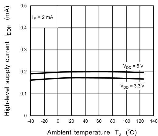
Fig. 13.2.8 I_{DDH} - T_a
