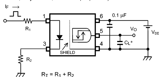
Fig. 13.1.5 Switching Time Test Circuit and Waveform
