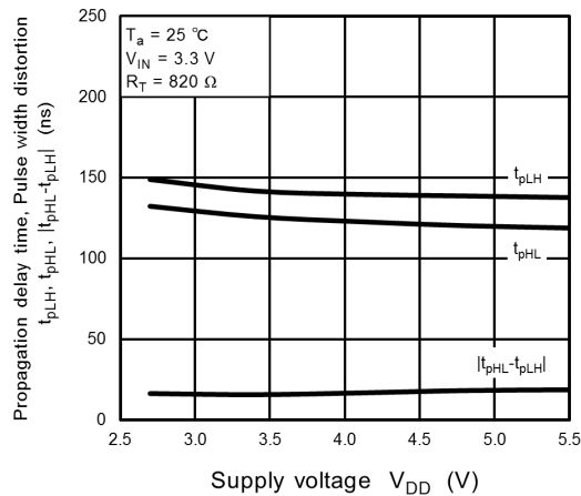
Fig. 13.2.13 t_{pLH} , t_{pHL} , |t_{pHL} - t_{pLH}| - V_{DD}
