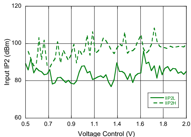
Input IP2 @ 2 GHz
