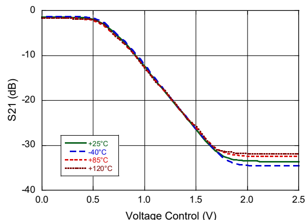
S21 @ 4 GHz
