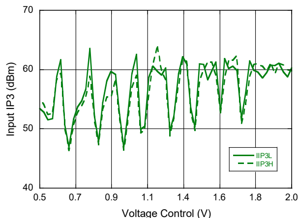
Input IP3 @ 2 GHz
