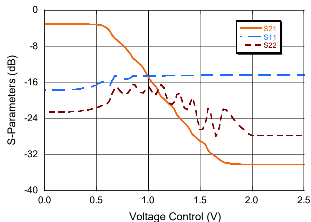
S21, S11, S22 @ 12 GHz
