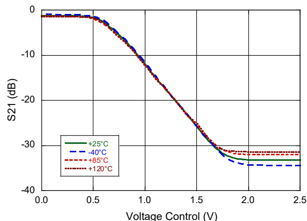
S21 @ 8 GHz
