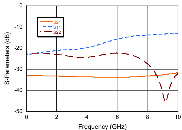
S11, S22, S21 @ V_C = 2.5\text{ V}
