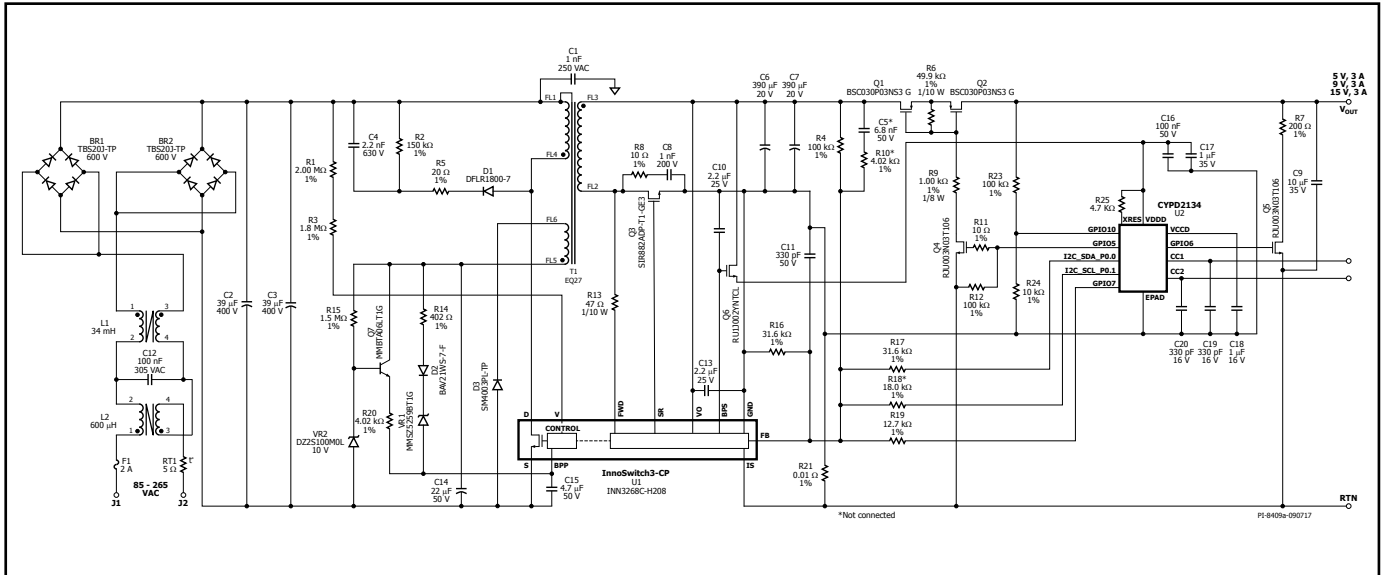
Figure 11. 5 V, 3 A ; 9 V, 3 A ; 15 V, 3 A USB PD 2.0 Compliant Adapter.
