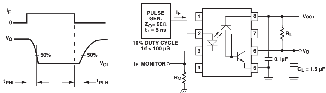
Figure 7. Switching test circuit.
