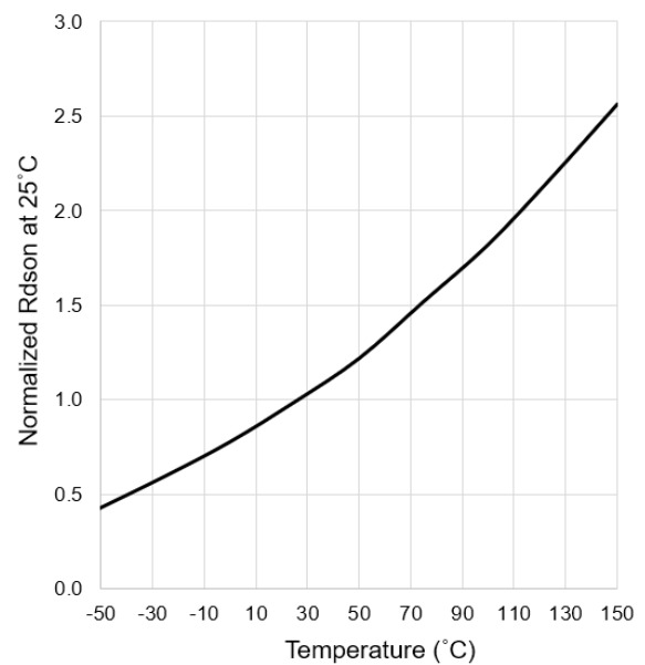
R_{DS(on)} Temperature Dependence
