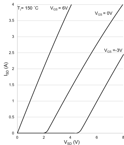
Figure 10: Typical I_{SD} vs. V_{SD} @ T_J = 150\text{ }^{\circ}\text{C}
