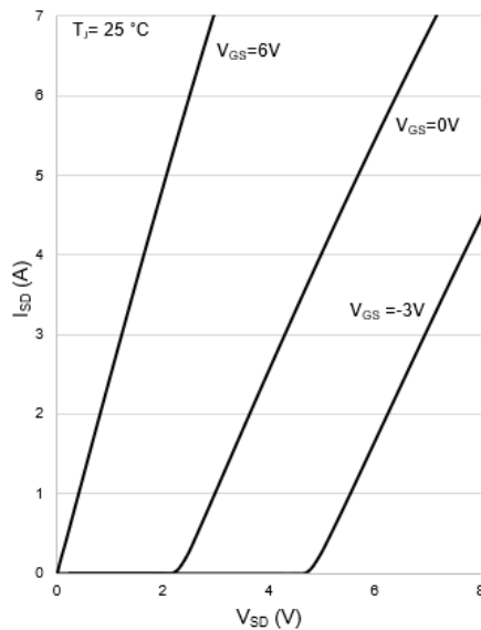
Reverse Conduction Characteristics
