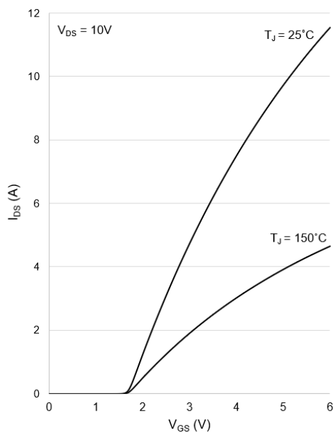
Figure 11: Typical I_{DS} vs. V_{GS}
