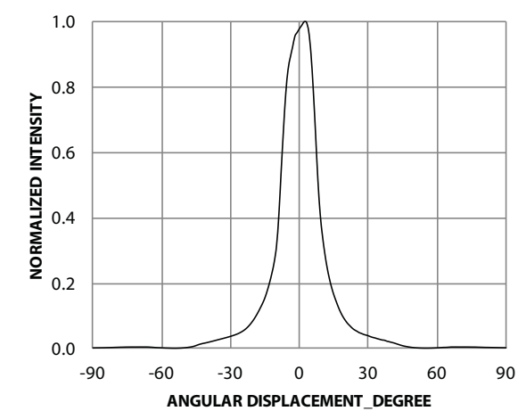
Figure 7: Radiation Pattern for X Axis for 15°
