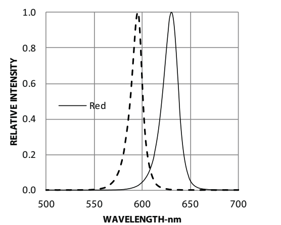
Figure 2: Relative Intensity vs. Wavelength
