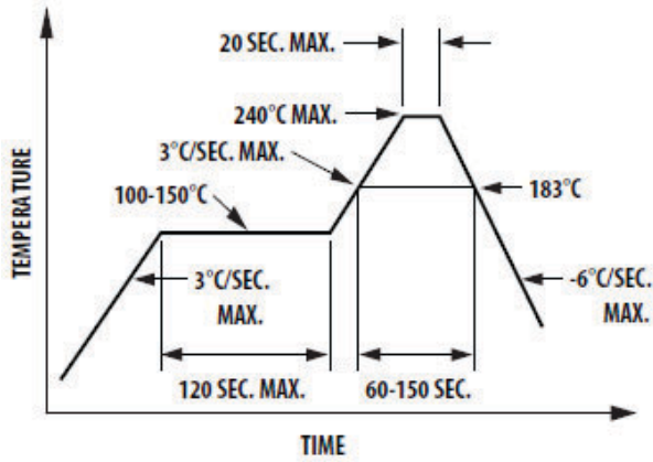
Figure 16: Lead Reflow Soldering
