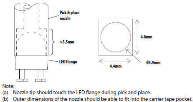
Figure 19: Nozzle Size
