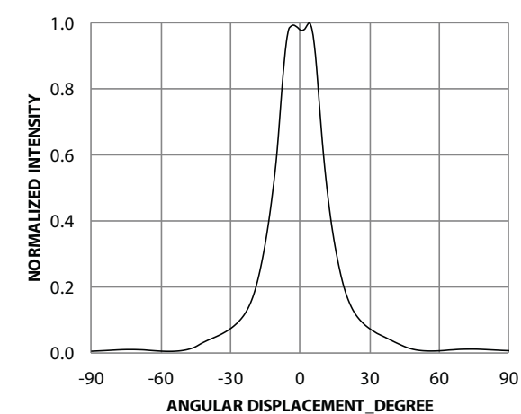
Figure 8: Radiation Pattern for X Axis for 23°
