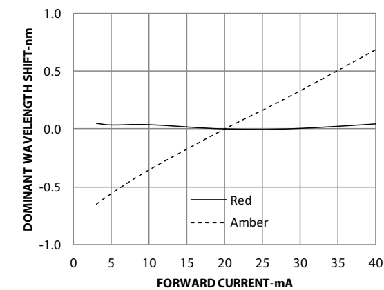
Figure 6: Relative Dominant Wavelength Shift vs. Forward Current
