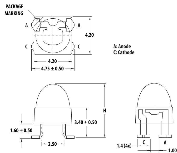
Figure 1: Package Dimensions
