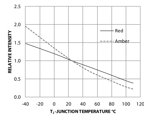
Figure 10: Relative Intensity vs. Junction Temperature
