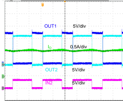
Time (20µs/div)
