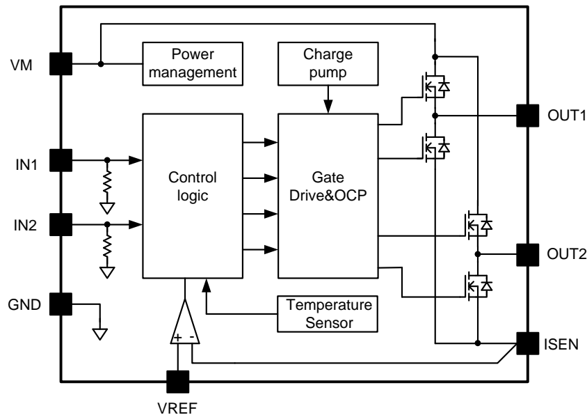
Figure2. Block Diagram
