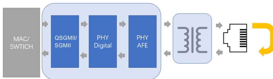
Figure 11. External Loopback
