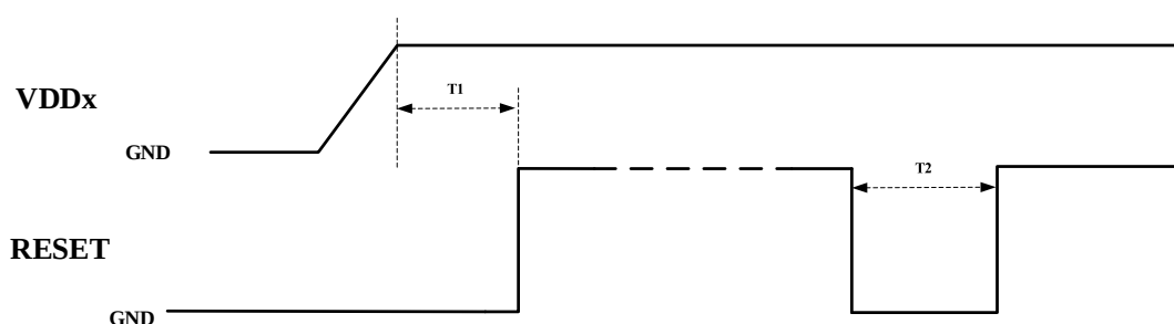
Figure 9. Reset Timing Diagram
