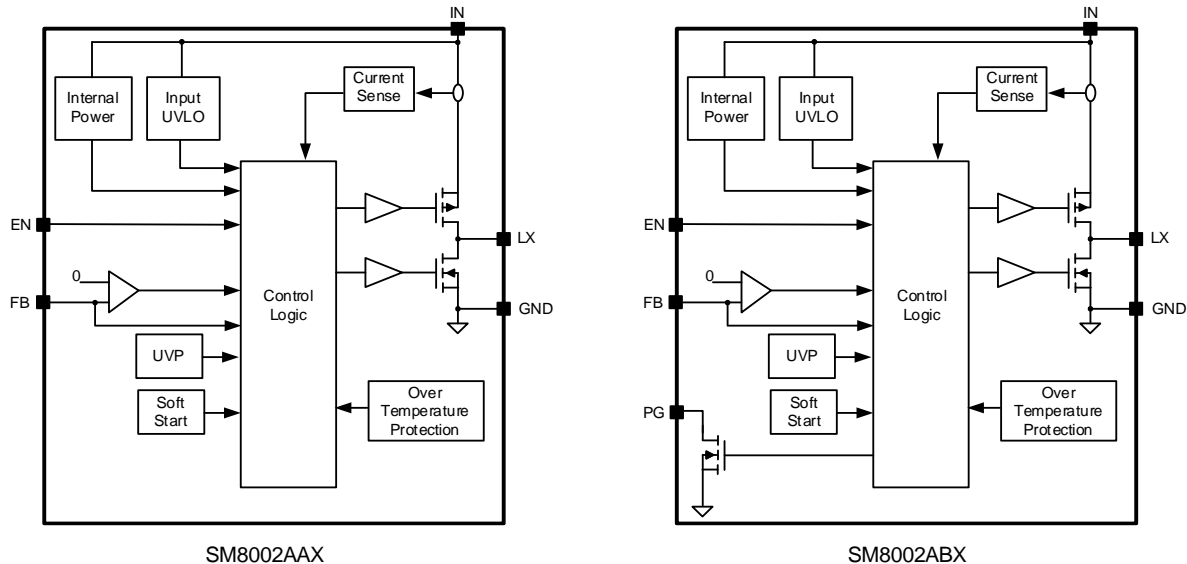
Figure3. Block Diagram
