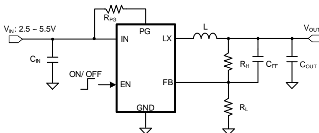
Figure 1. Schematic Diagram
