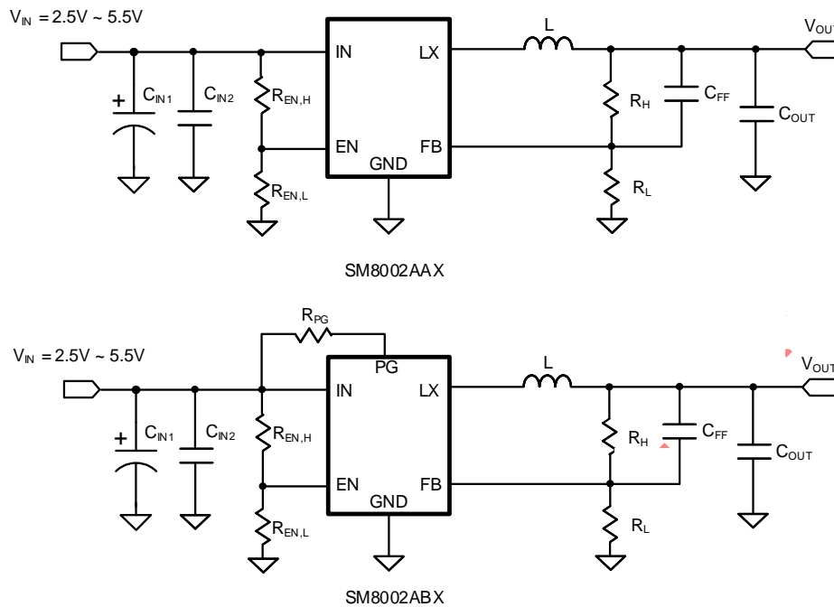
Figure6. Schematic Diagram
