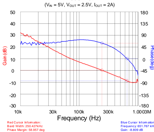
Bode Plot
