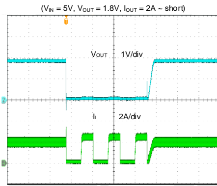
Time 4ms/div
