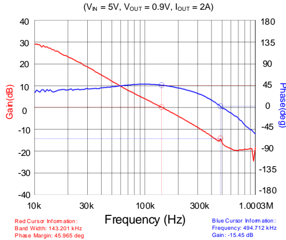
Bode Plot
