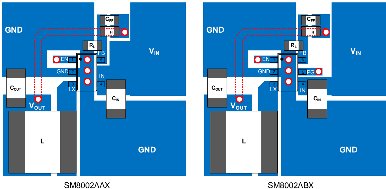
Figure 7. Suggested PCB Layout
