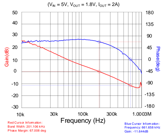
Bode Plot
