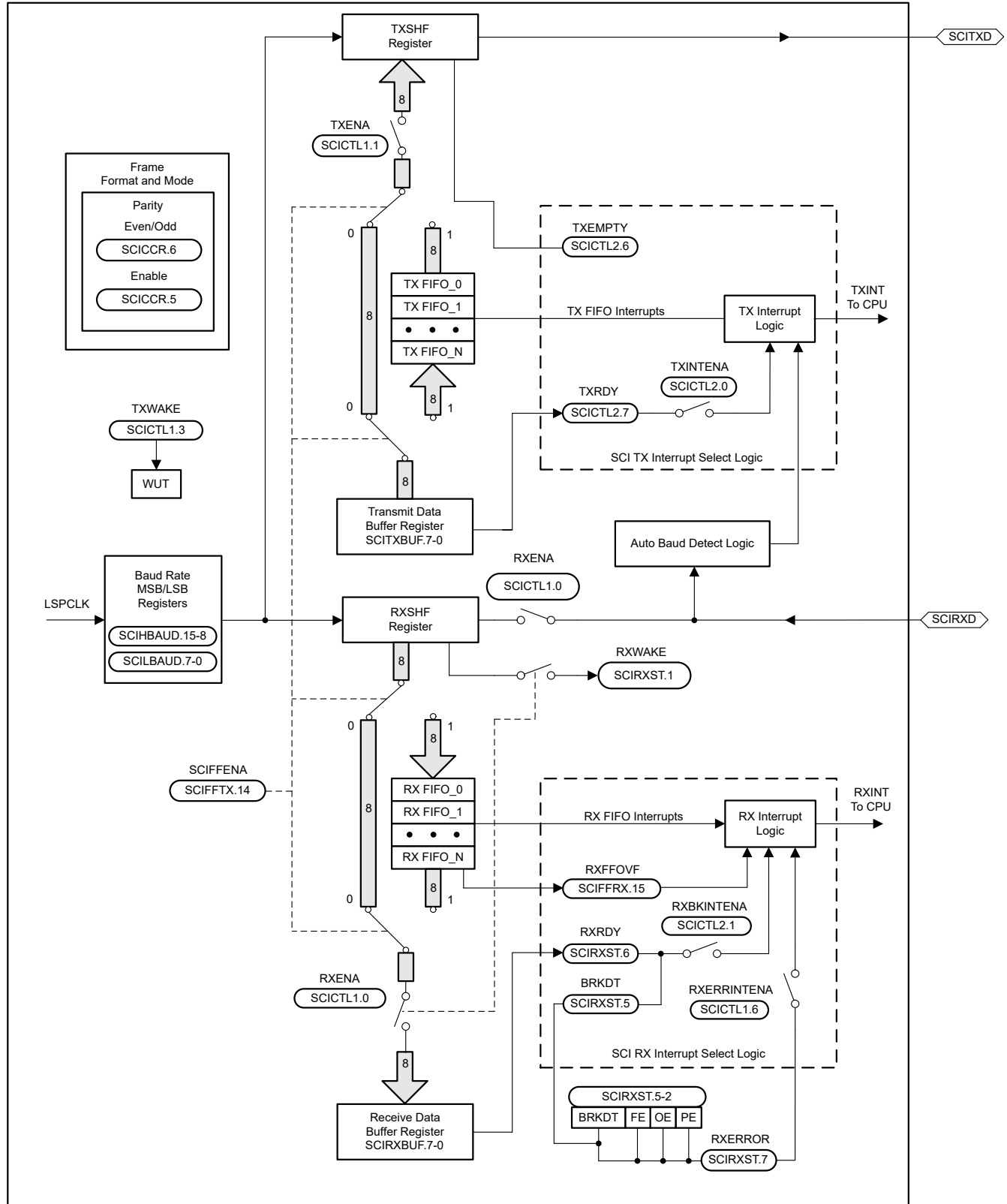
Figure 6-68. SCI Block Diagram
