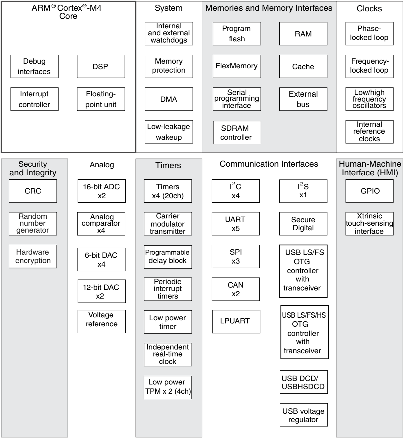
Figure 1. K26 Block Diagram
