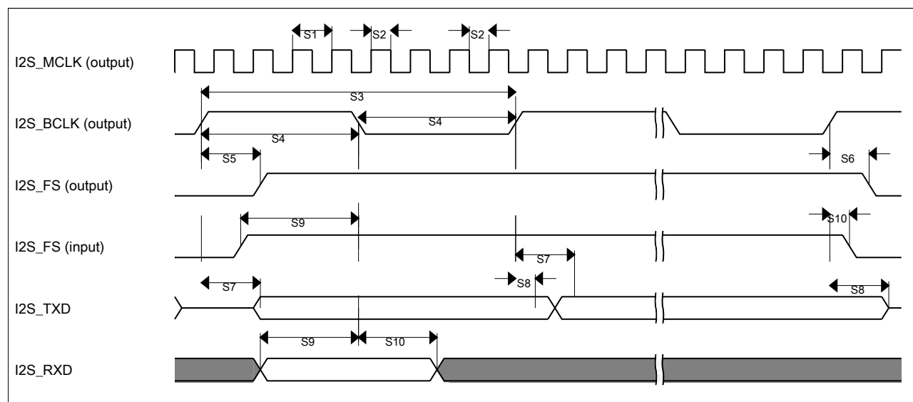
Figure 29. I 2 S timing — master mode
