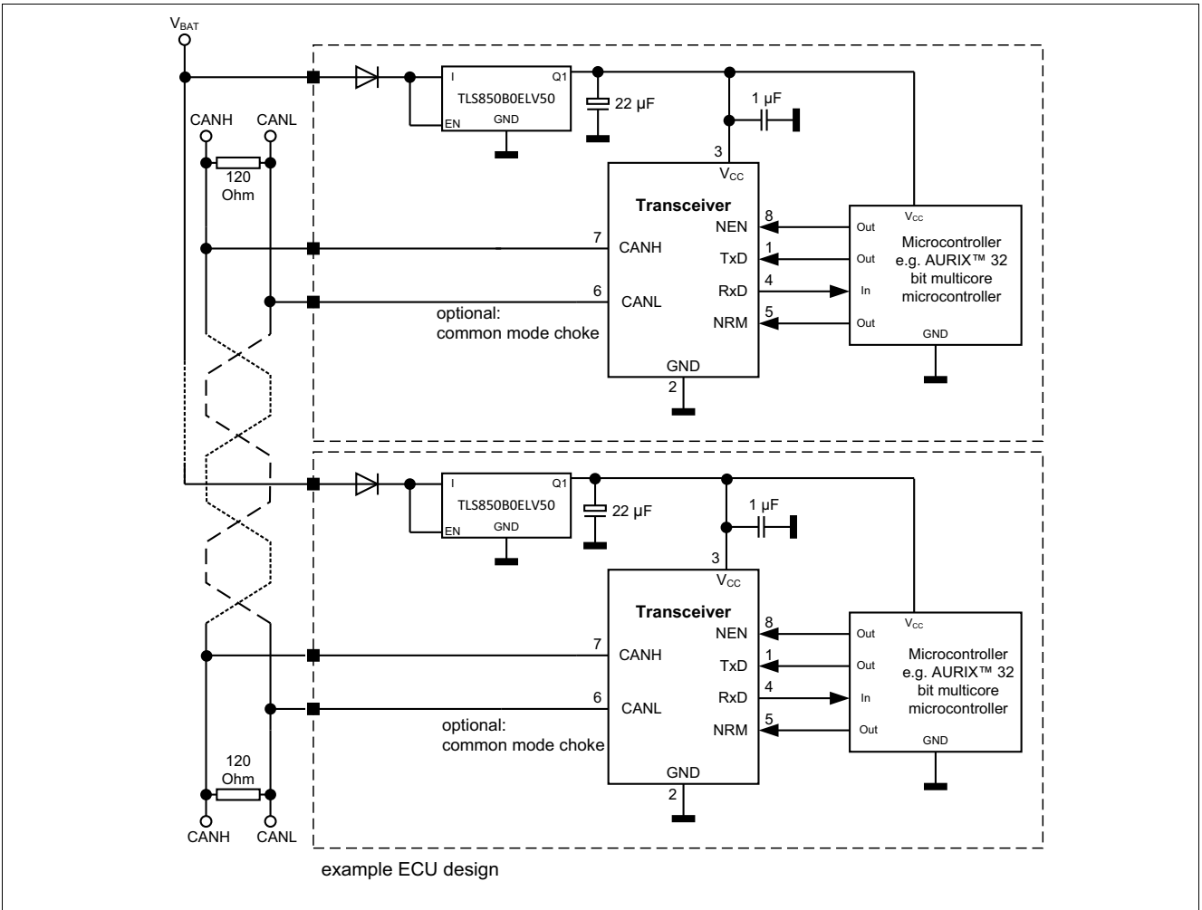
Figure 11 Application circuit
