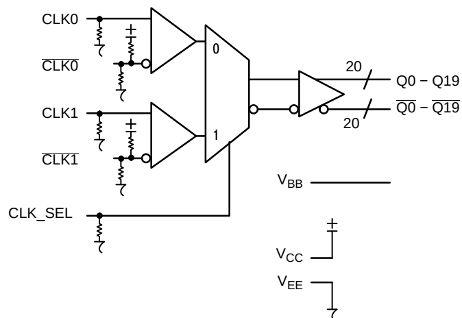
Figure 2. Logic Diagram
