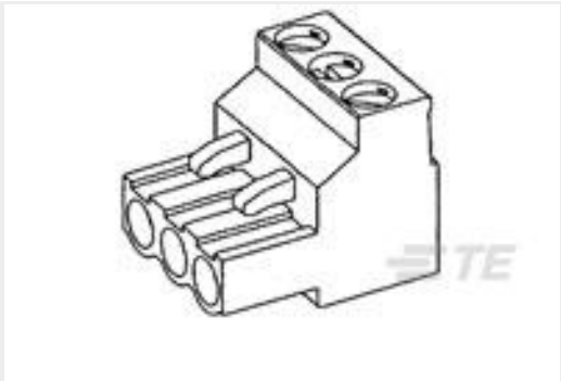
TE Part #1-796981-2 12POS TERMI-BLOK R/A PLUG 7.62
