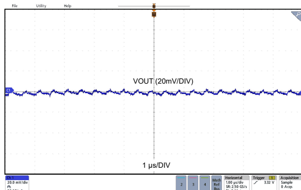
LMQ66430MC3 V_{OUT} = 3.3V 2A 负载 修复
