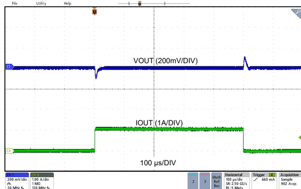
LMQ66430MC3 V_{OUT} = 3.3V 2.2MHz (FPWM) 0A 至 1A, 1A/ \mu s 修复
