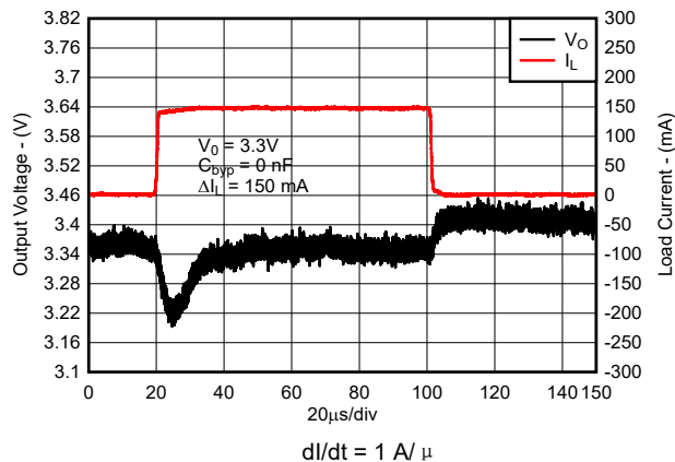
图 7-8. Load Transient Response for New Chip
