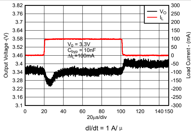
图 7-4. Load Transient Response for New Chip
