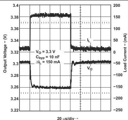
图 7-3. Load Transient Response for Legacy Chip
