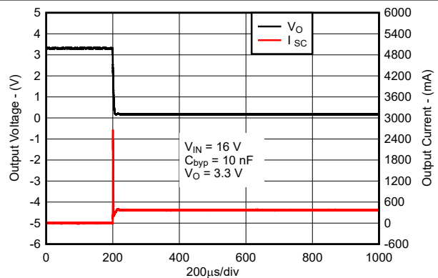
图 5-10. Short-Circuit Current vs Time for New Chip
