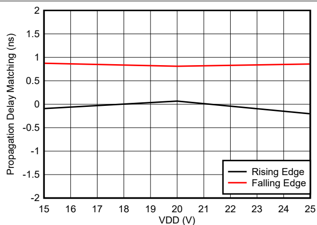
Figure 5-14. Propagation Delay Matching (t DM ) vs VDD
