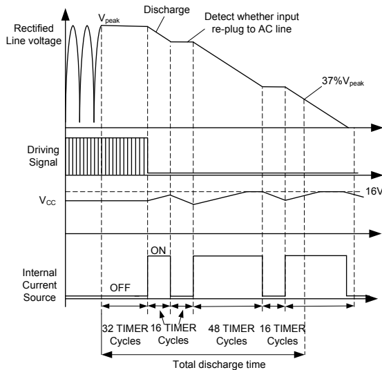
Figure 10: X-Cap Discharger
