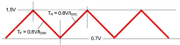
Figure 6: Voltage Profile of TMR
