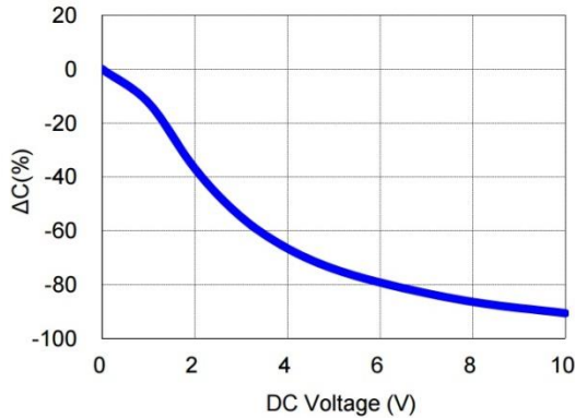
Figure 16. C EFF for 22 µF, 0603, X5R, 10 V-Rated Capacitor (SEMCO CL10A226MP8NUNE)
