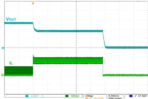
Figure 14. Overload Protection
