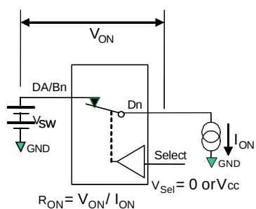
Figure 4. On Resistance
