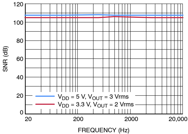
Figure 13. Signal-to-Noise Ratio vs. Frequency, R_L = 2.5\text{ k}\Omega
