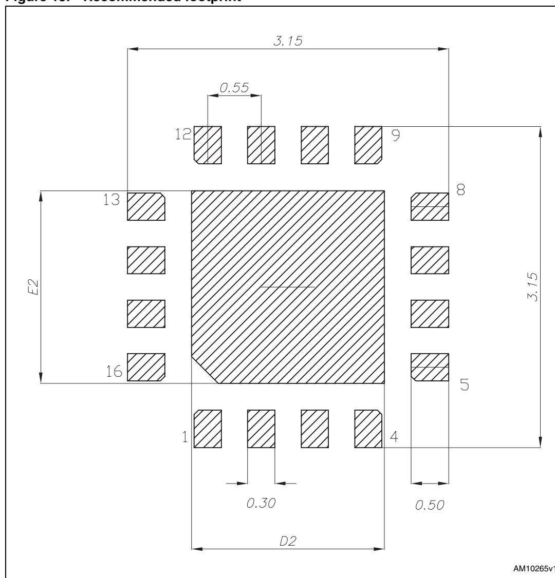
Figure 15. Recommended footprint
