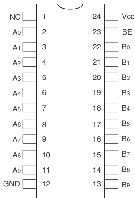
QSOP/ TSSOP TOP VIEW
