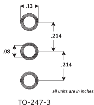
TO-247-3
