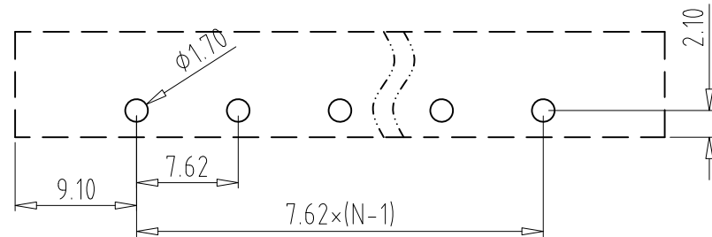
PCB LAYOUT
