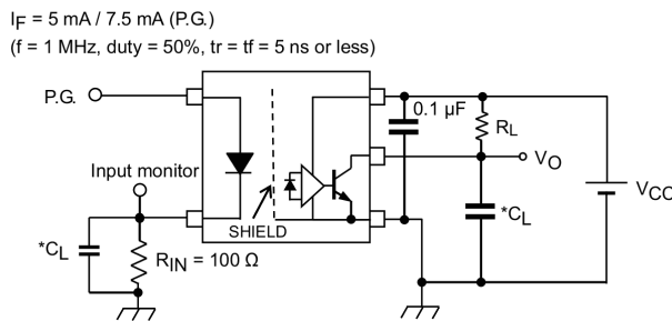
Fig. 12.1.3 ICCL Test Circuit
