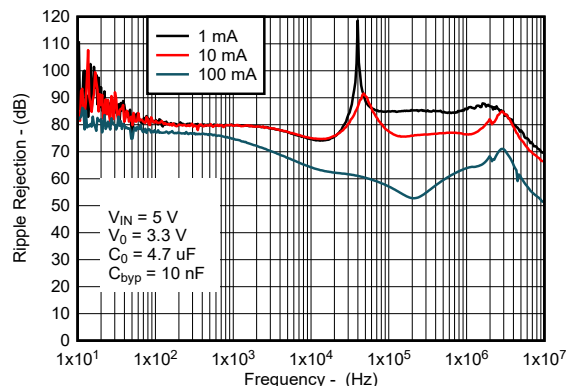
Figure 5-25. Ripple Rejection vs Frequency for New Chip
