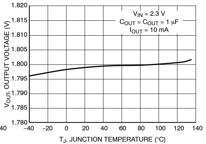
Figure 58. Output Voltage vs. Temperature V_{OUT} = 1.8\text{ V}
