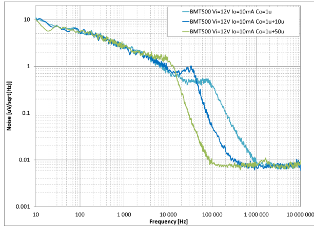
Figure 49. Noise – FIX – 5.0 V, I_{OUT} = 10\text{ mA} , Different C_{OUT}
