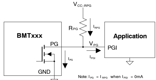
Figure 81. Circuit Example for R_{PG} Value Selection
