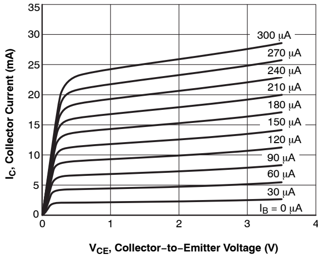
Figure 1. I_C - V_{CE}
