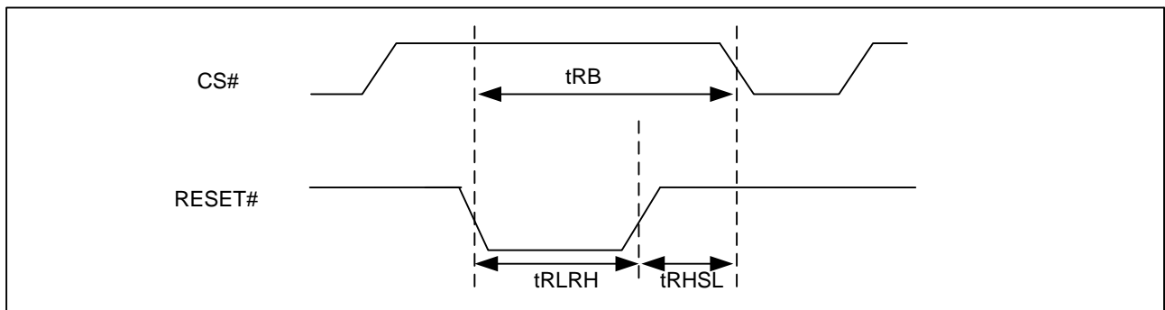
Figure82. RESET Timing
