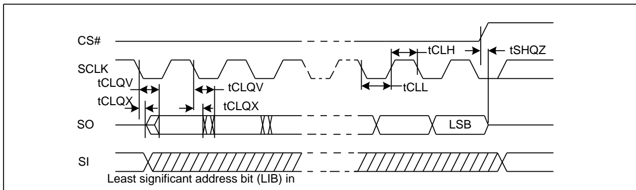
Figure 79. Output Timing
