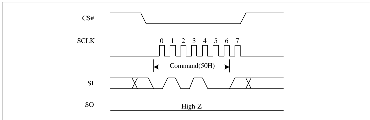
Figure 7. Write Enable for Volatile Status Register Sequence Diagram
