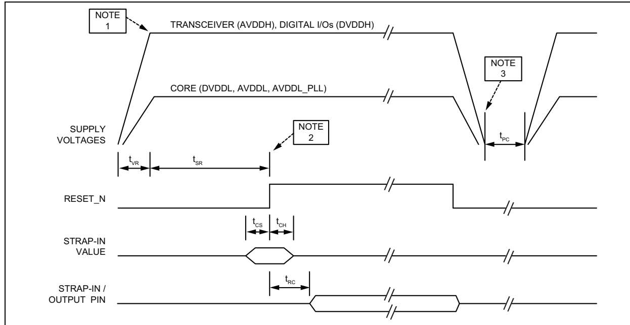
FIGURE 7-7: POWER-UP/POWER-DOWN/RESET TIMING
