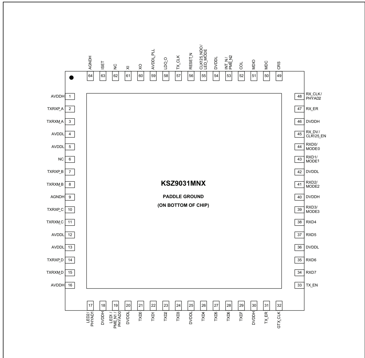
FIGURE 2-1: 64-QFN PIN ASSIGNMENT (TOP VIEW)
