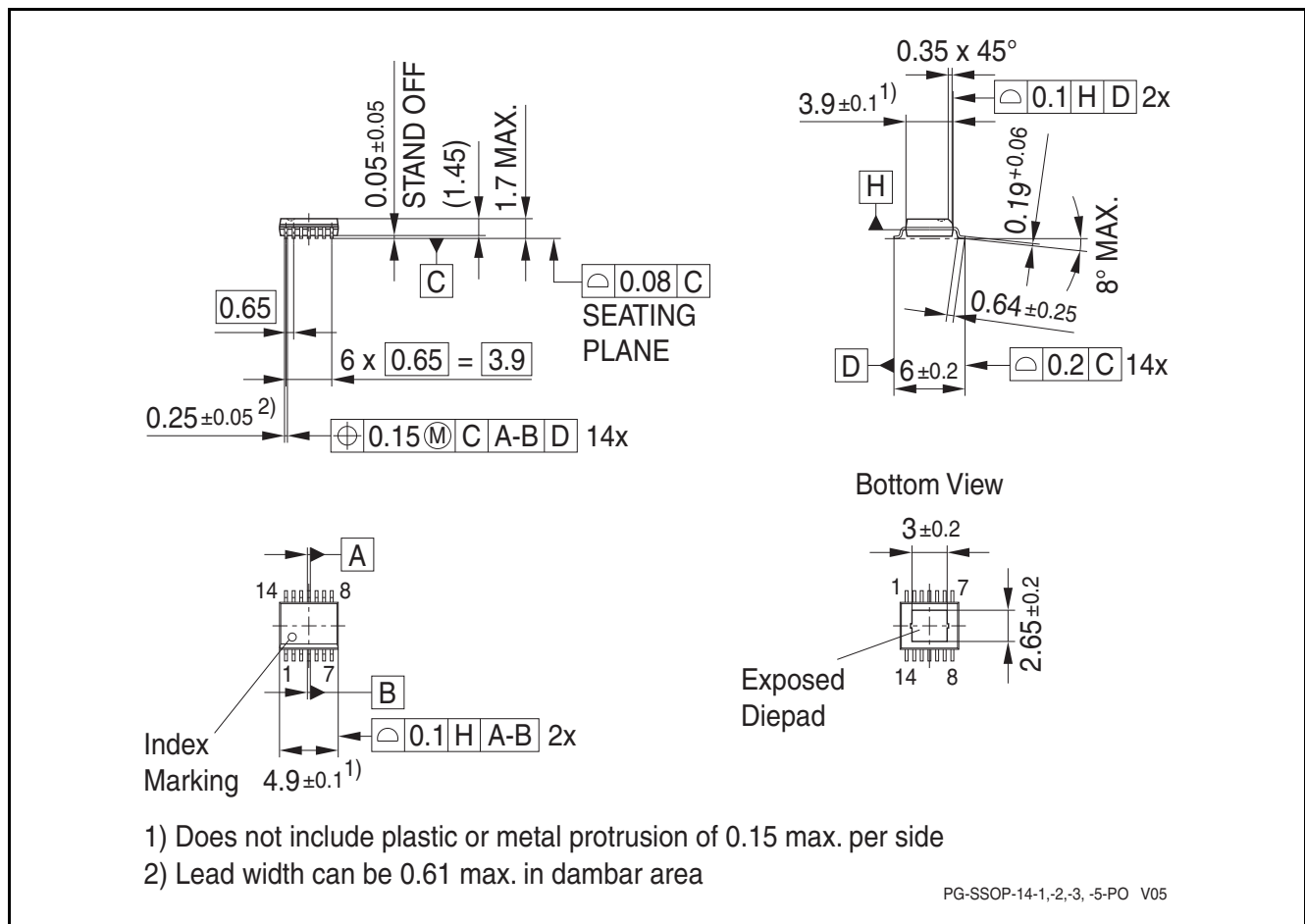
Figure 32 Outline PG-SSOP-14-3
