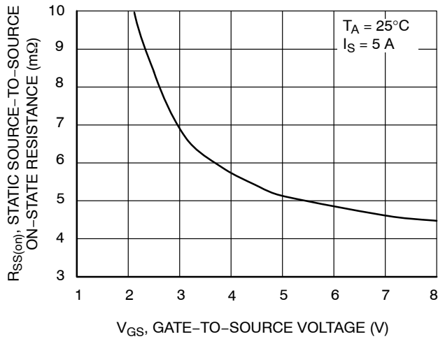
Figure 10. R_{SS(on)} - V_{GS}
