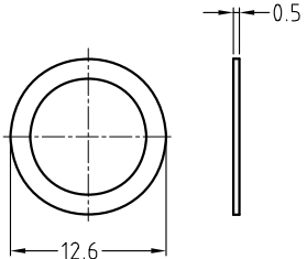
METAL WASHER
