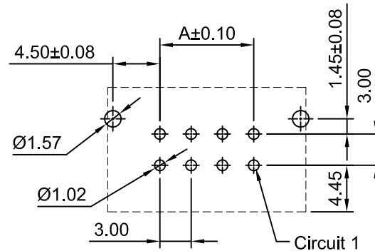
P.C.B LAOUT (TOP VIEW) TOLERANCE:±0.05
