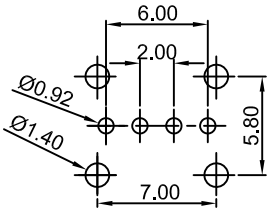
Recommend PCB layout (Tolerance:±0.05)
