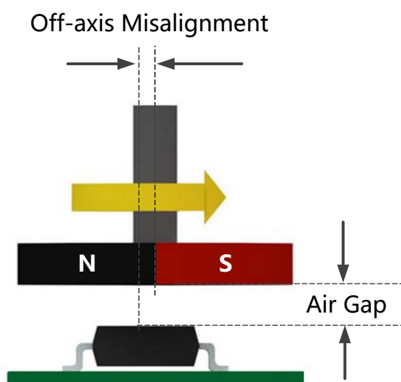
Figure 4: Magnet Arrangement
