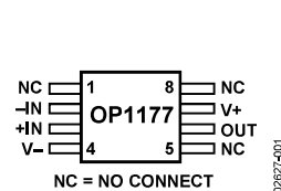
Figure 1. 8-Lead MSOP (RM Suffix)
