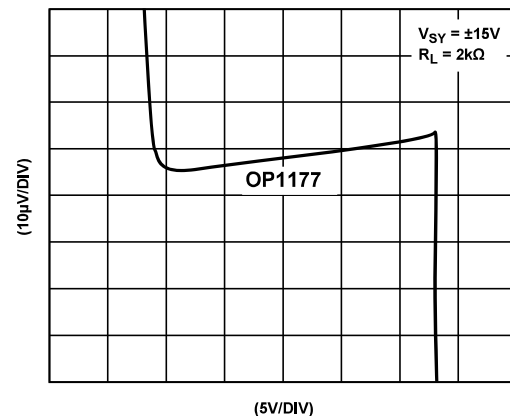
Figure 51. Gain Linearity
