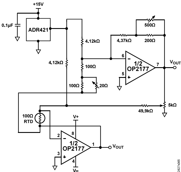
Figure 65. Low Power Linearized RTD Circuit
