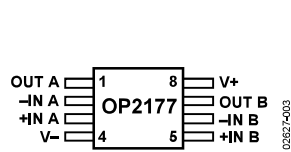
Figure 3. 8-Lead MSOP (RM Suffix)
