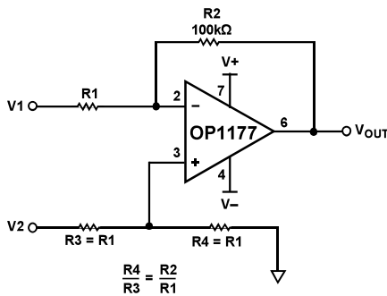
Figure 63. Difference Amplifier
