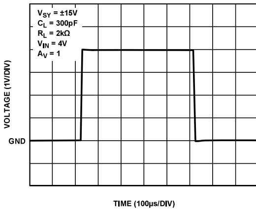
Figure 15. Large Signal Transient Response
