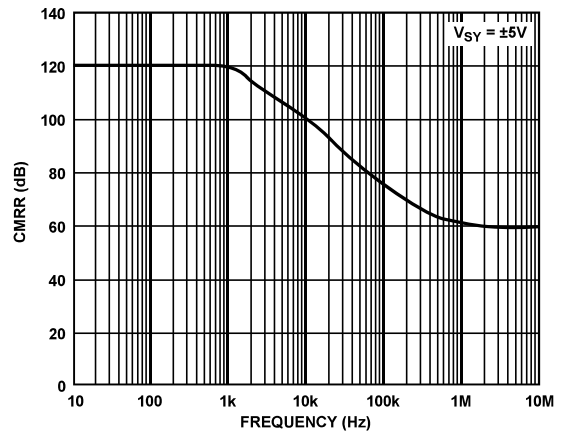
Figure 41. CMRR vs. Frequency
