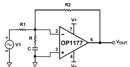
Figure 62. Compensation Using Input R-C Network
