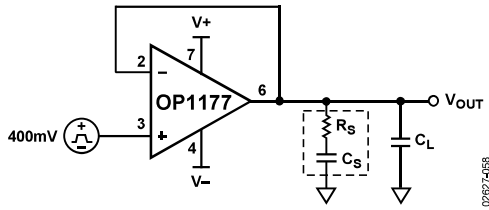
Figure 58. Snubber Network Configuration
