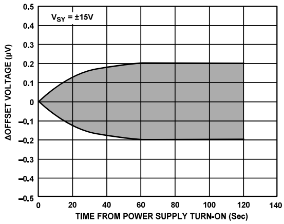
Figure 26. Warm-Up Drift
