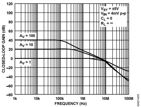
Figure 33. Closed-Loop Gain vs. Frequency
