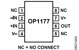
Figure 2. 8-Lead SOIC_N (R Suffix)
