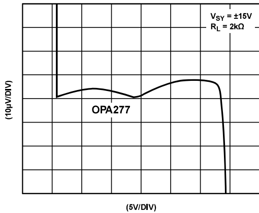
Figure 52. Gain Linearity
