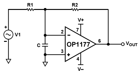
Figure 61. EMI Reduction
