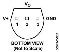
Figure 3. 3-Lead TO-92
