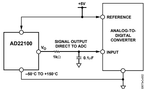
Figure 2. Application Circuit
