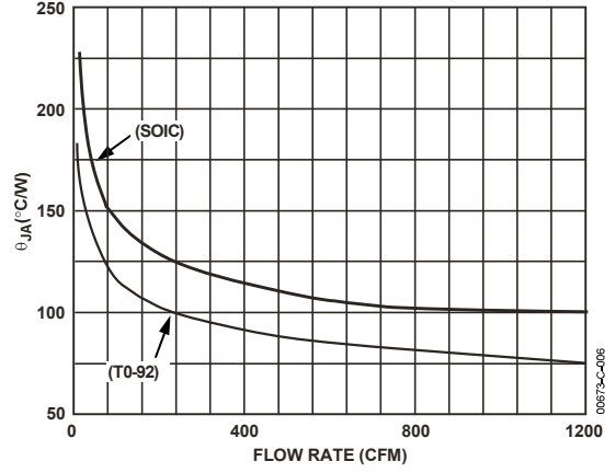
Figure 6. Thermal Resistance vs. Flow Rate
