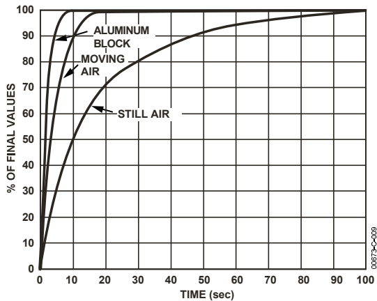
Figure 10. Response Time
