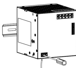
⑤ Turn the Phillips screwdriver to the left to loosen the terminal screws, insert the head of the wire into the bottom of the terminal, and then turn the screwdriver to the right to tighten the terminal screws
