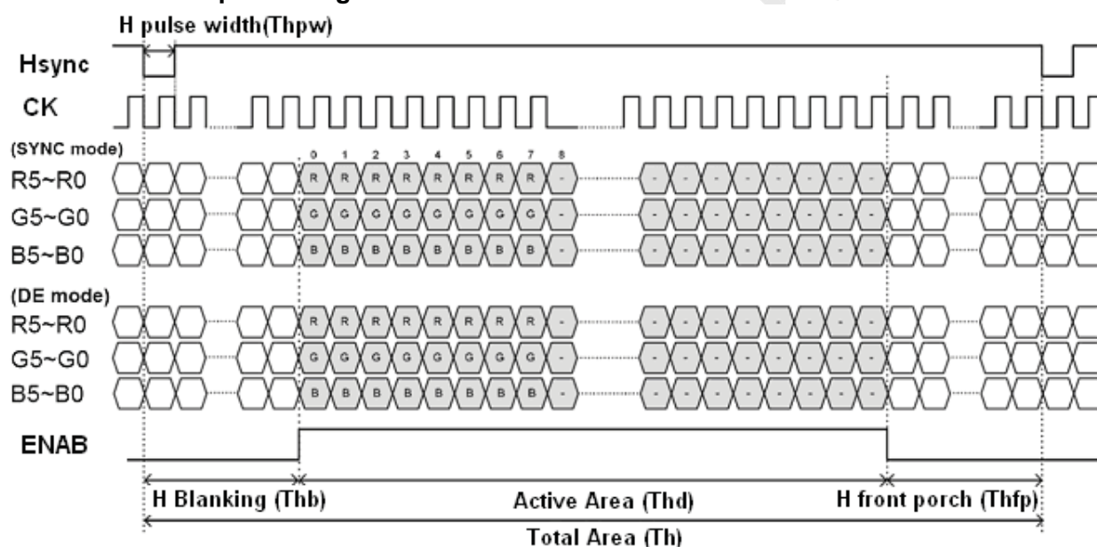
Figure 5.3.2 Horizontal input timing
