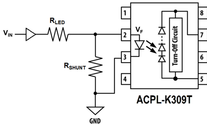
Figure 16: Input Circuit
