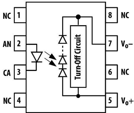
Figure 1: ACPL-K309T Functional Diagram
