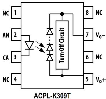
Figure 3: ACPL-K309T Pinout
