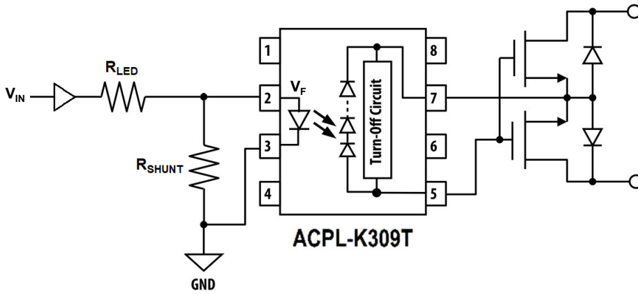
Figure 2: Application Circuit
