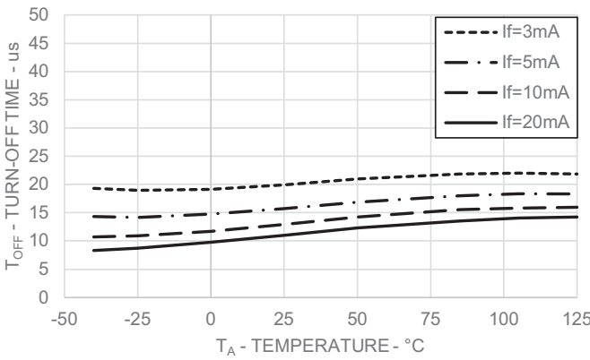
Figure 13: Turn-Off Time vs. Operating Temperature (at C_L = 1\text{ nF} )
