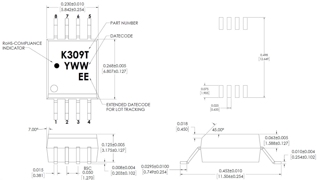
Figure 4: Stretched SO-8 Package
