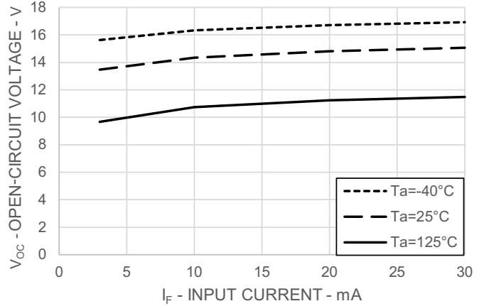
Figure 6: Open-Circuit Voltage vs. Input Current
