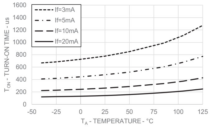
Figure 12: Turn-On Time vs. Operating Temperature (at C_L = 1\text{ nF} )
