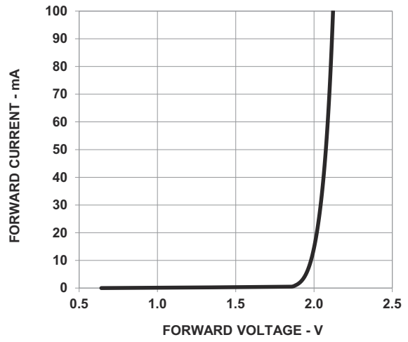
Figure 7: Forward Current vs. Forward Voltage
