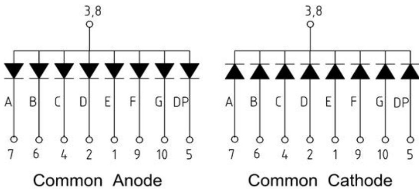
Figure 2: Circuit Diagram
