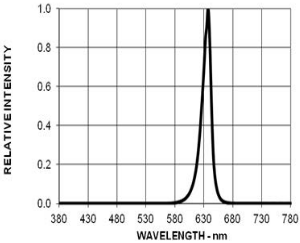
Figure 5: Relative Luminous Intensity vs. Wavelength
