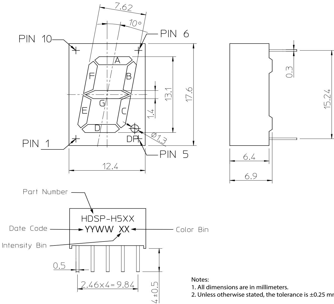
Figure 1: Package Dimensions
