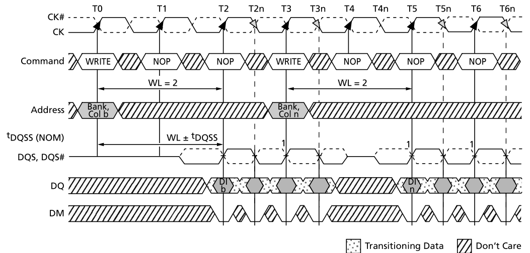
Figure 60: Nonconsecutive WRITE-to-WRITE
