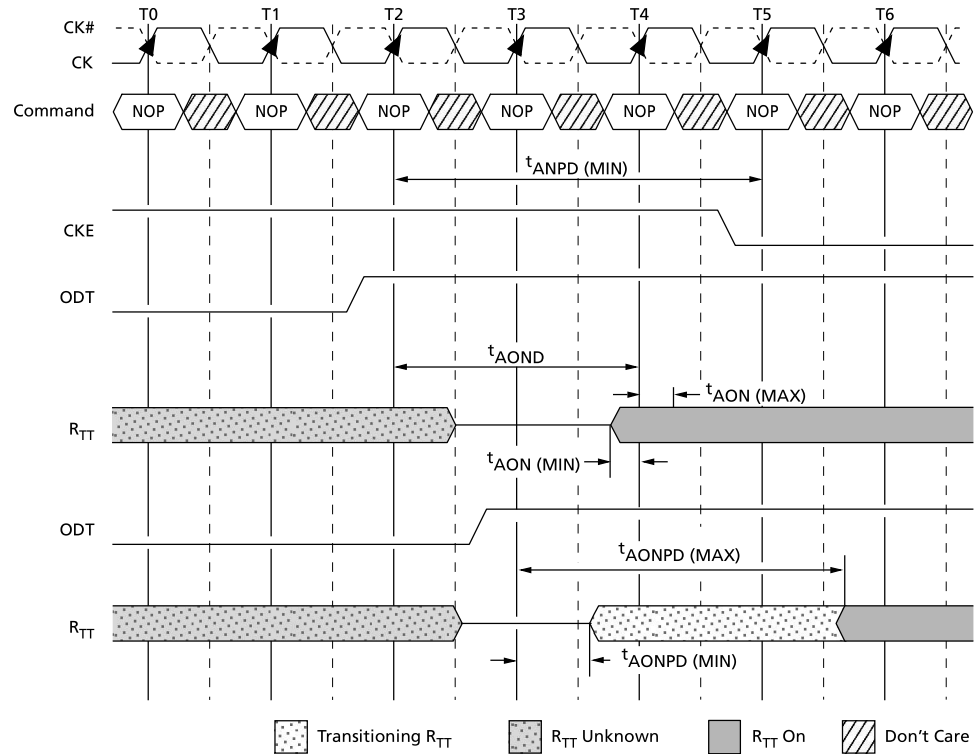
Figure 86: ODT Turn-On Timing When Entering Power-Down Mode
