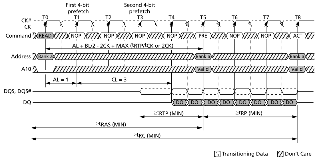
Figure 52: READ-to-PRECHARGE – BL = 8
