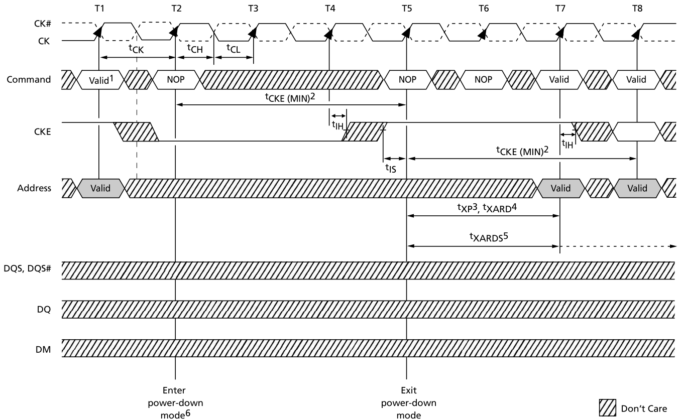
Figure 70: Power-Down
