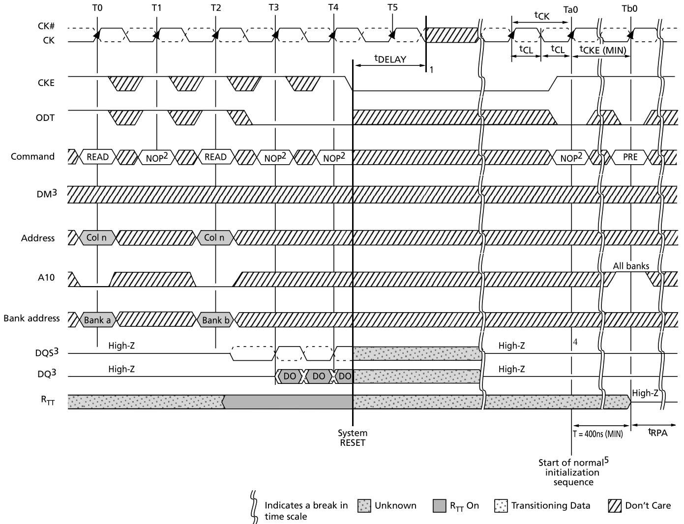
Figure 80: RESET Function
