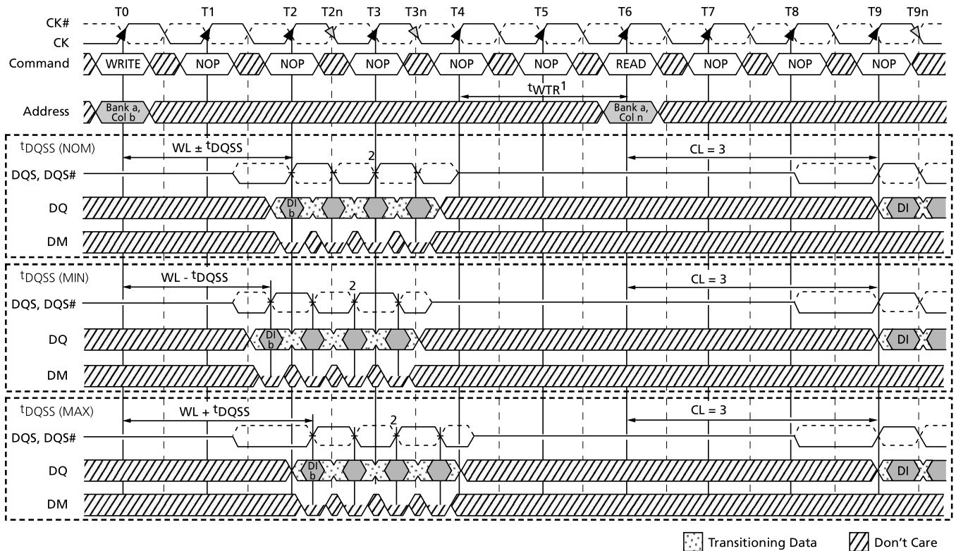
Figure 62: WRITE-to-READ
