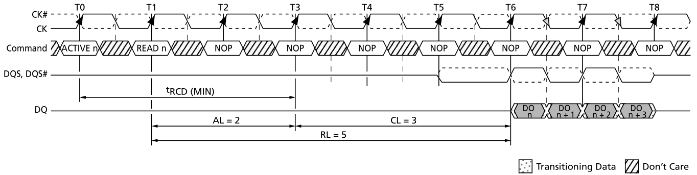
Figure 39: READ Latency
