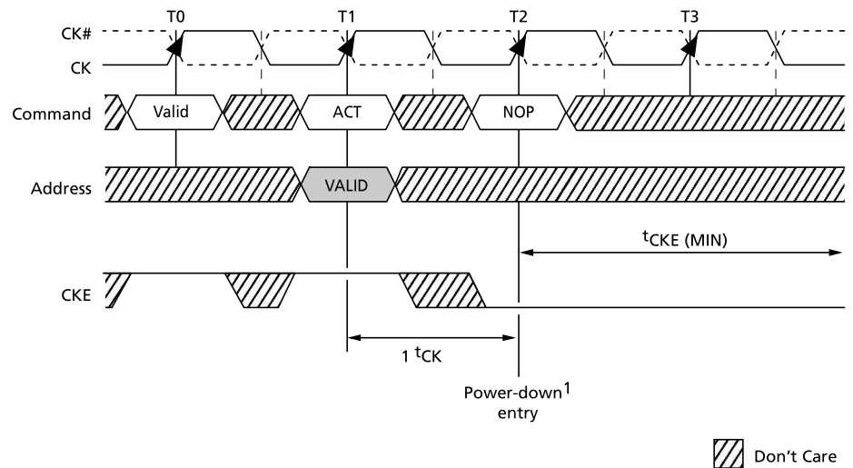
Figure 76: ACTIVATE Command-to-Power-Down Entry
