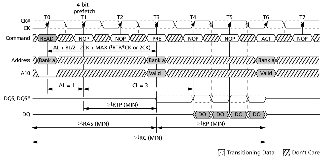
Figure 51: READ-to-PRECHARGE – BL = 4
