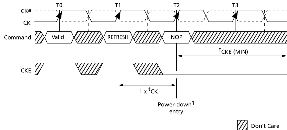
Figure 75: REFRESH Command-to-Power-Down Entry
