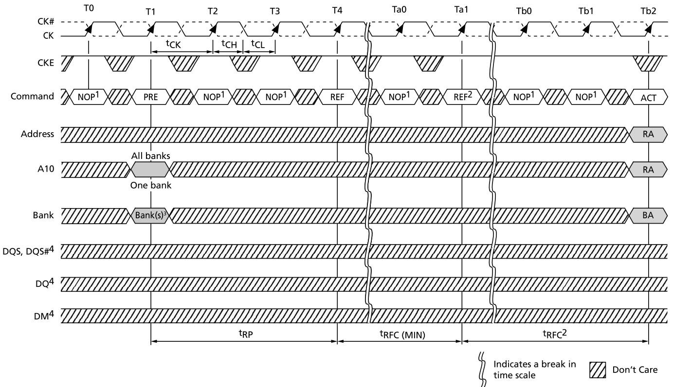
Figure 68: Refresh Mode
