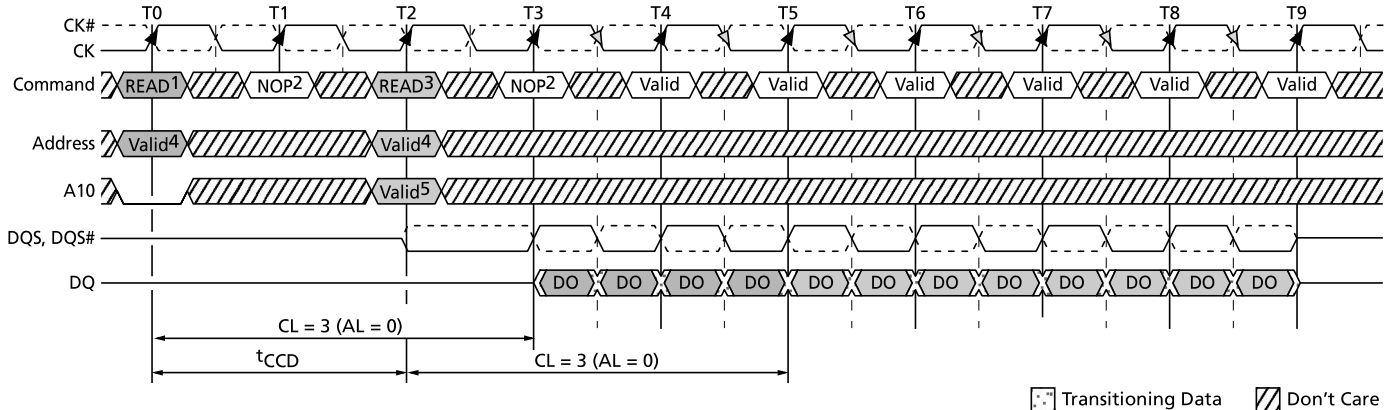
Figure 49: READ Interrupted by READ
