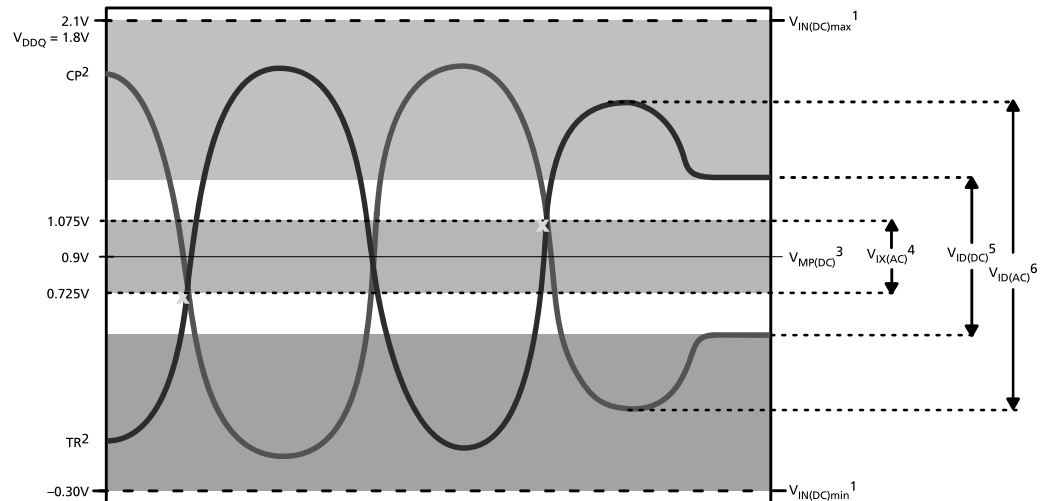
Figure 14: Differential Input Signal Levels
