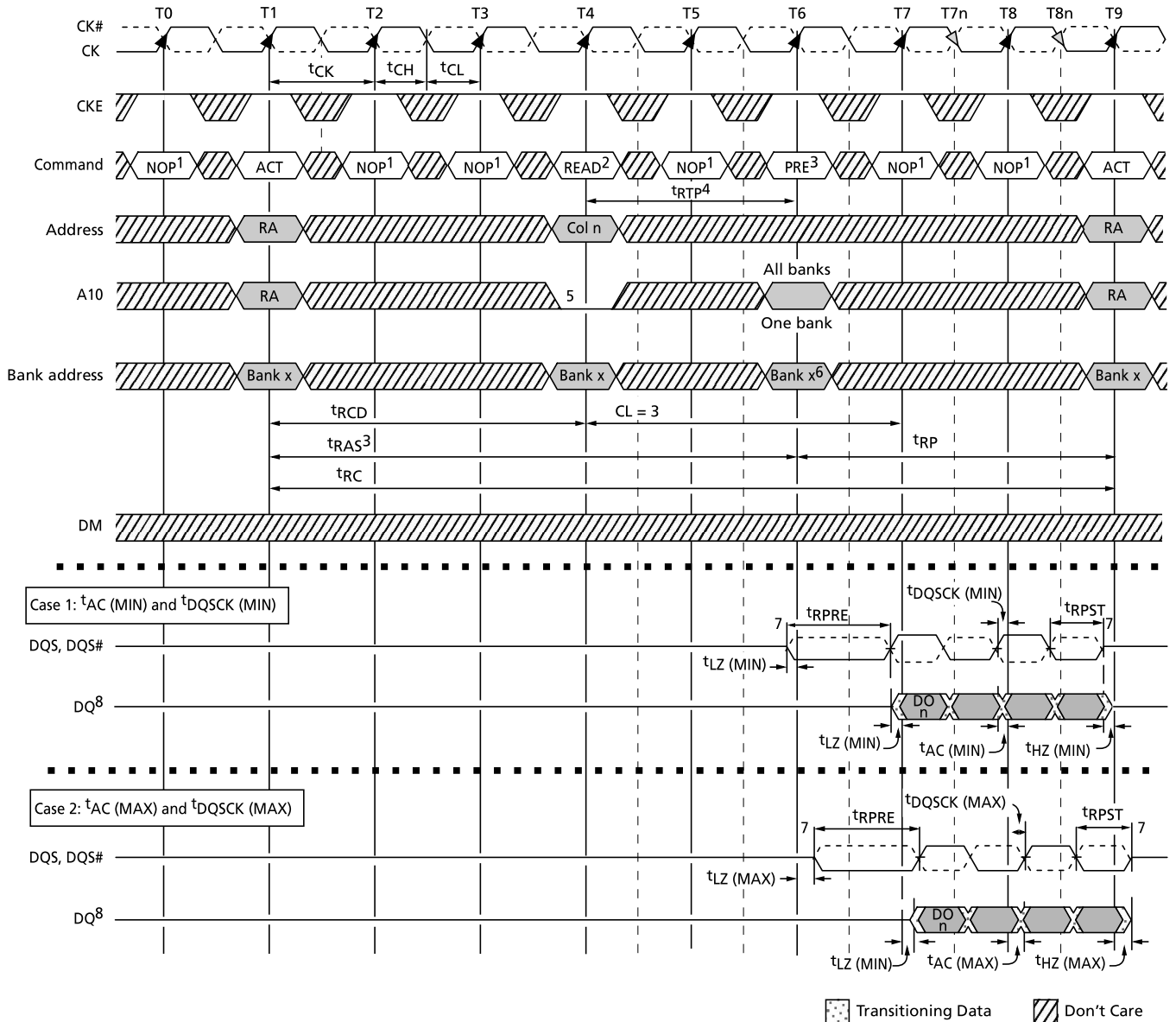
Figure 53: Bank Read – Without Auto Precharge
