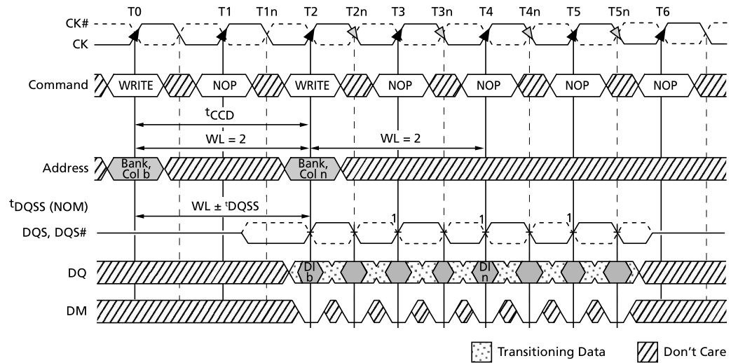
Figure 59: Consecutive WRITE-to-WRITE
