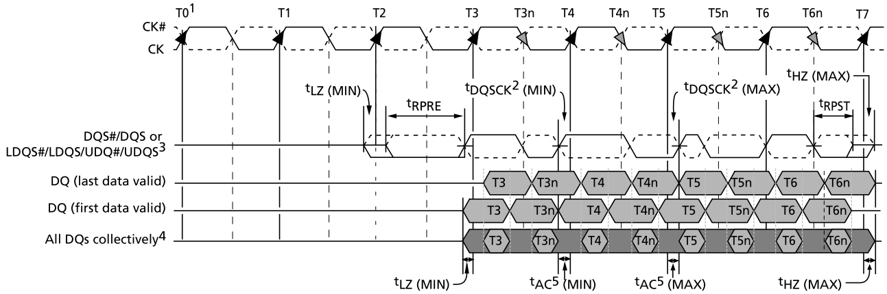
Figure 57: Data Output Timing – t_{AC} and t_{DQSK}
