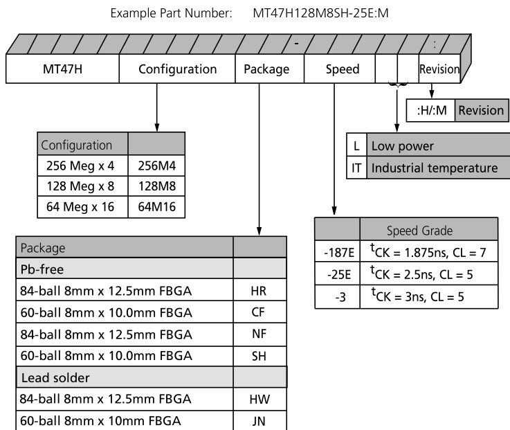
Figure 1: 1Gb DDR2 Part Numbers
