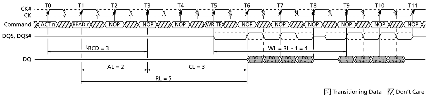
Figure 50: READ-to-WRITE
