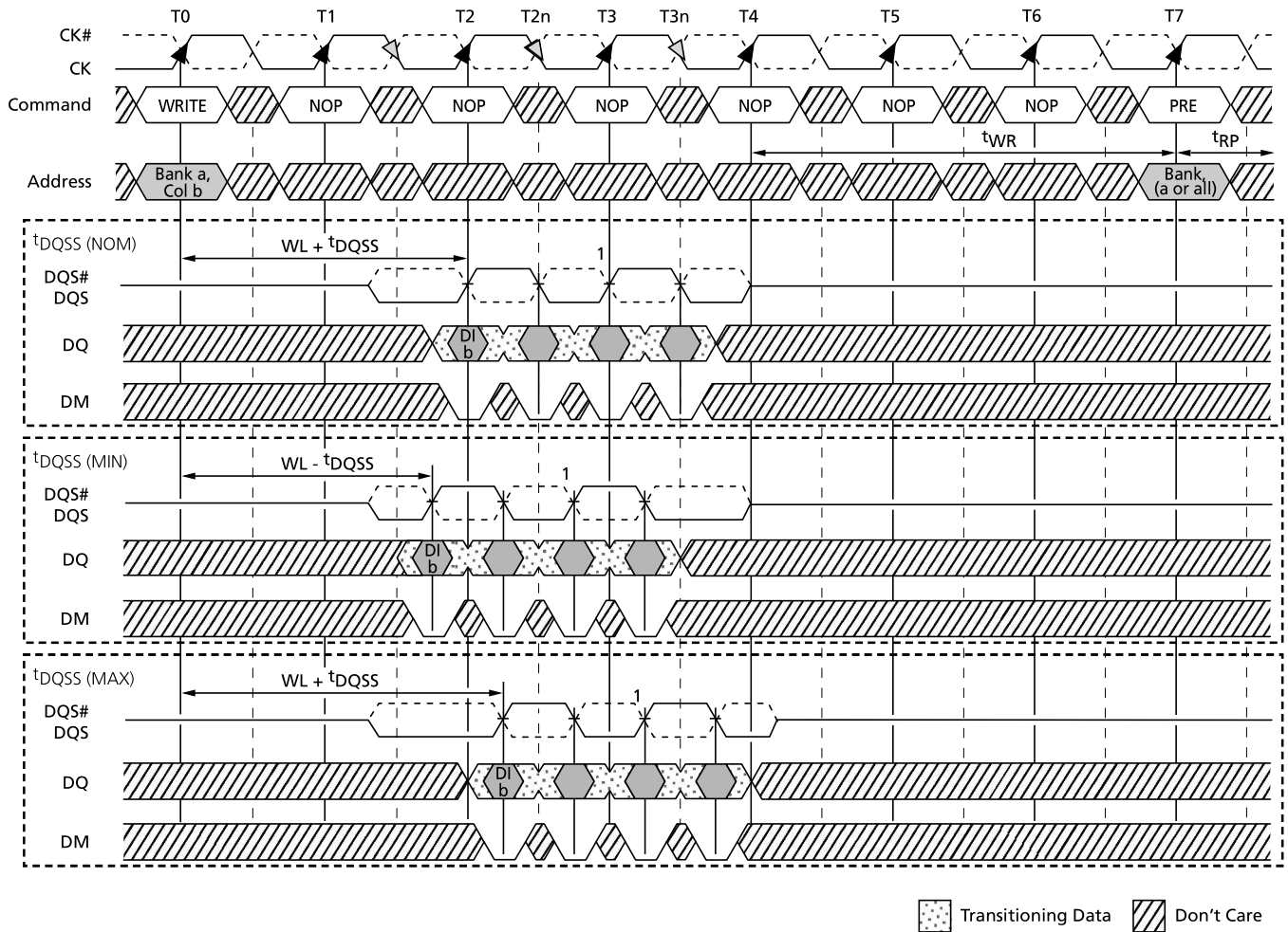
Figure 63: WRITE-to-PRECHARGE
