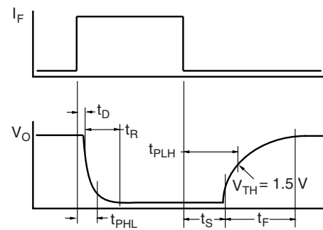
Fig. 13 - Switching Timing
